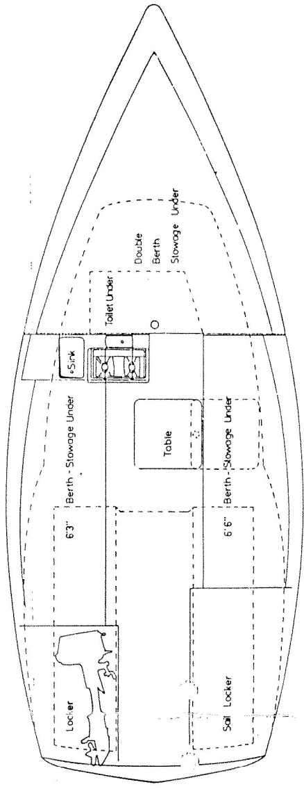
INTERIOR PLAN
