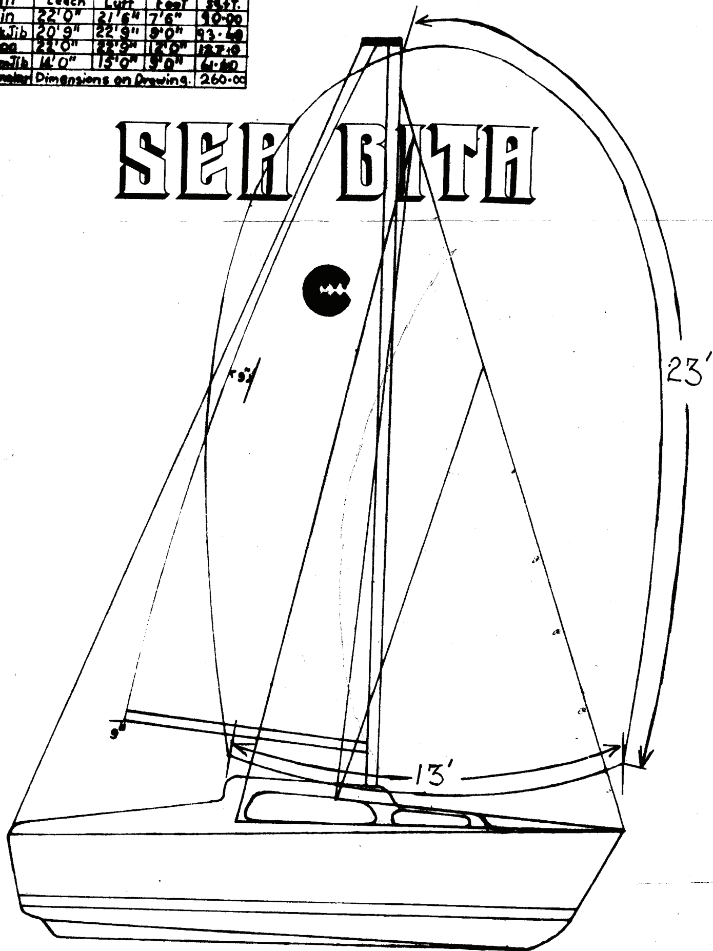
Sail plan for SEA BITA class trailer-sailer Sources and provided courtesy of John Crawford Marine 2012
